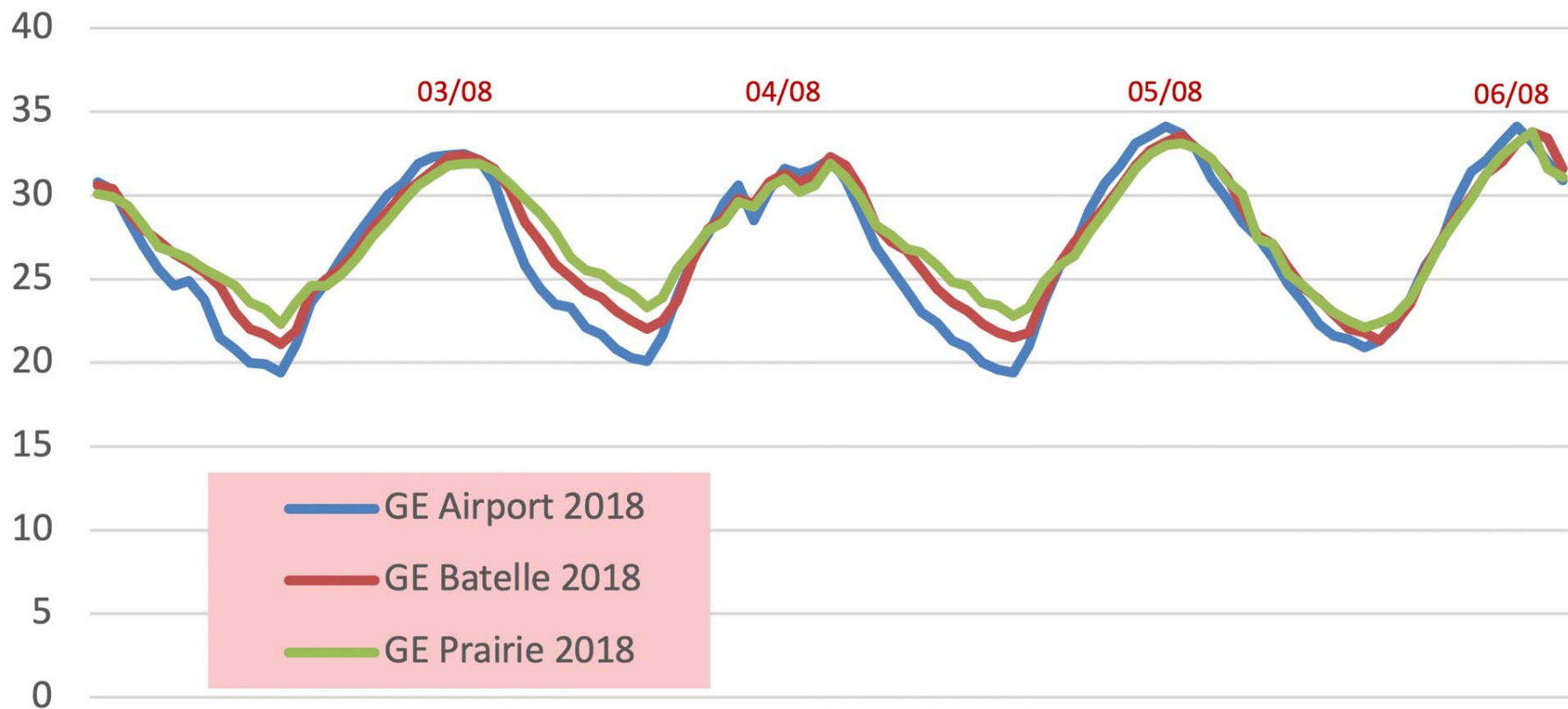
Temperatures in 3 Geneve City Locations in August 2018
